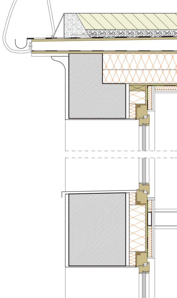
VERTICAL CROSS SECTION THROUGH FACADE WITH WINDOW AND DOOR WINDOW IN INTERNAL INSULATION LINE
