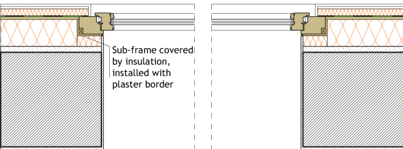
HORIZONTAL CROSS SECTION THROUGH FACADE WITH INTERNAL INSULATION
