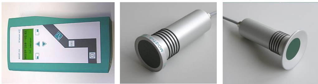
Figure 53: Example of a microwave moisture analyser with different measuring heads (Source: hf-sensor.de)
