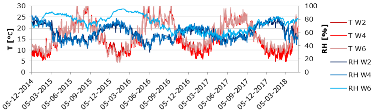
Figure 33: Relative humidity and temperature between insulation and historic wall construction measured in the case study building in Meinungsgade, Copenhagen. Relative humidity shows strong fluctuations, which are untypical for a construction with a vapour barrier.
