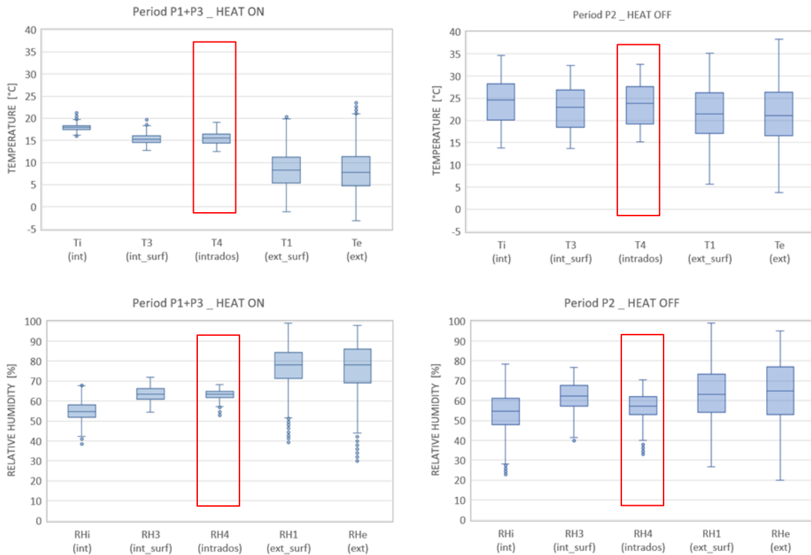
Figure 29: Temperature (upper graphs) and relative humidity (lower graphs) conditions for the heating season (left graphs) and for the free-running season (right graphs) in the RIBuild case study building Villa Graciosi in Ancona.
