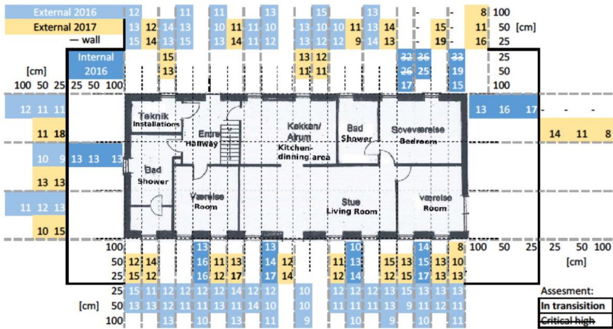
Figure 56: Troxler measurements before insulating and again after insulating. The first values in a double column (shown with faded and thick dashed line) contain 2016 and 2017 measurements (e.g. upper left:12, 13, 15 & 12, 14) measured in the middle of the covered wall length while the following single column include 2016 and 2017 measurements (e.g. upper left: 14, 13 & 15, 13) below the window. The third column only include measurements from 2016. Heights stated are measured from the foundation. Yellow boxes are placed where possible due to space limitations. Values from 17 to 25 are assessed as in transition between non-critical and critical moisture content for bricks while above 25 is critical.
