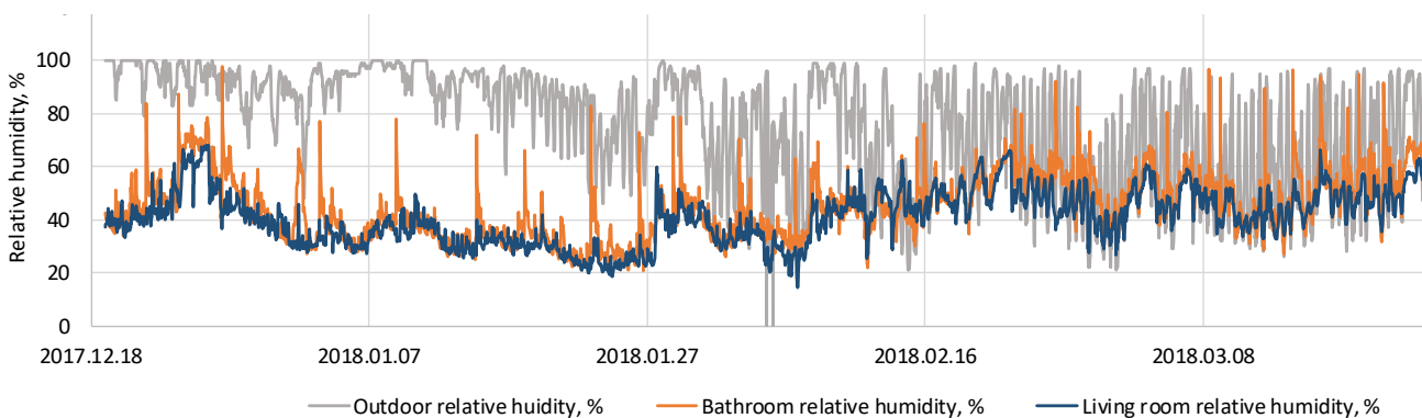
Figure 28: Outdoor and indoor relative humidity for two rooms in the test case building in Dankepi, Latvia. The values for the bathroom are on the average on a typical level but show regular peaks due to the usage
