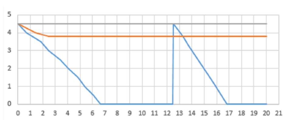
Figure 59: Water uptake test results (Karsten tube) from RIBuild case study building Spikeri, Riga (Latvia): the paint has peeled off due to humidity influence (blue line), plain layer of paint 1 m above the point with peeled paint (orange line) and plain layer of paint (grey line). Y-scale gives the scale of the Karsten tube water column, X-scale gives the time in minutes.
