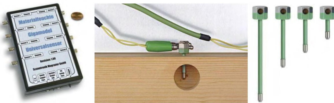
Figure 52: 8-fold extension module, measuring cables and electrodes to measure moisture content in masonry and rendering.
