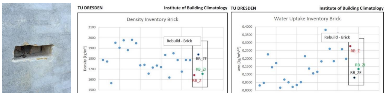
Figure 1: Sample extraction (left picture) from the case study building in Klütgaarden, Denmark. Diagrams in the middle and on the right show results of the laboratory measurements. Named dots in the frame are three different bricks extracted from Klütgaarden building, showing a huge variety of values.
